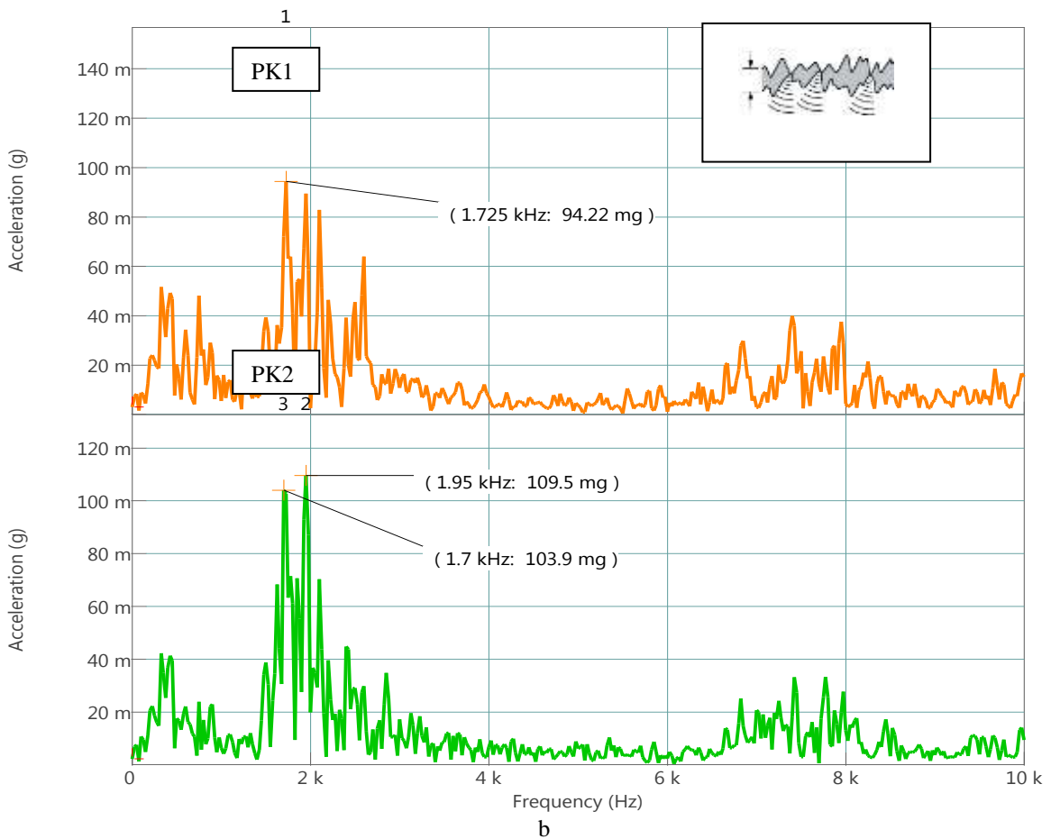
Fig.5 Vibration acceleration spectra with grease lubricant (a) and without grease lubricant (b) bearing without preloads F_1=0 N: PK1 transducer output upper and PK2 transducer output lower plots
