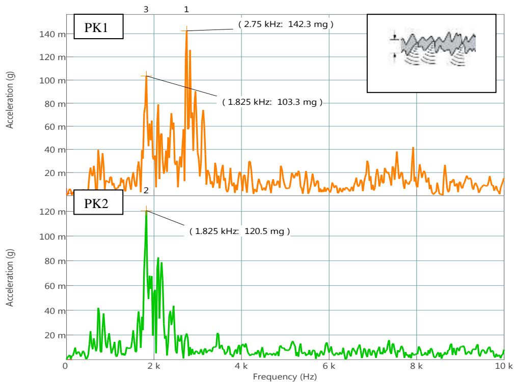
Fig. 4 Vibration acceleration spectra with grease lubricant (a) and without grease lubricant (b), with preloads F_1=100 N: PK1 transducer output upper and PK2 transducer output lower plots
